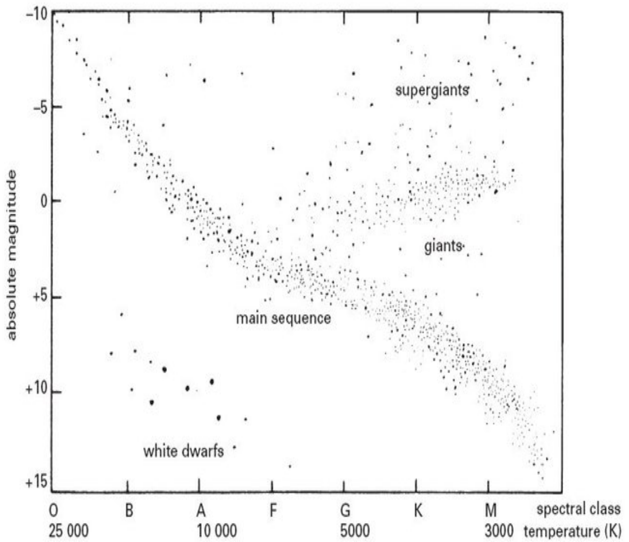
Hertzsprung-Russell diagram
