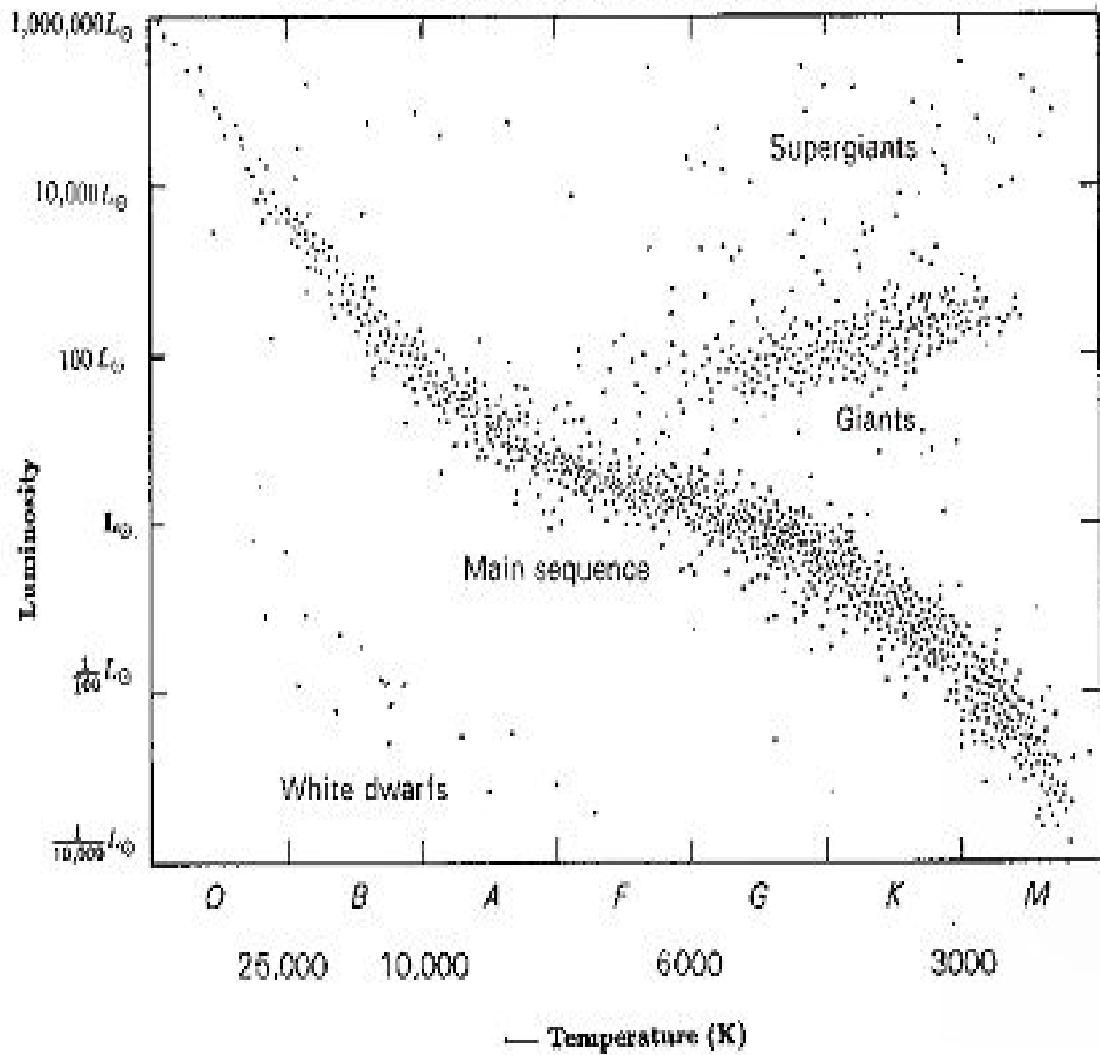
Hertzsprung-Russell Diagram for Stars in the Solar Neighborhood
